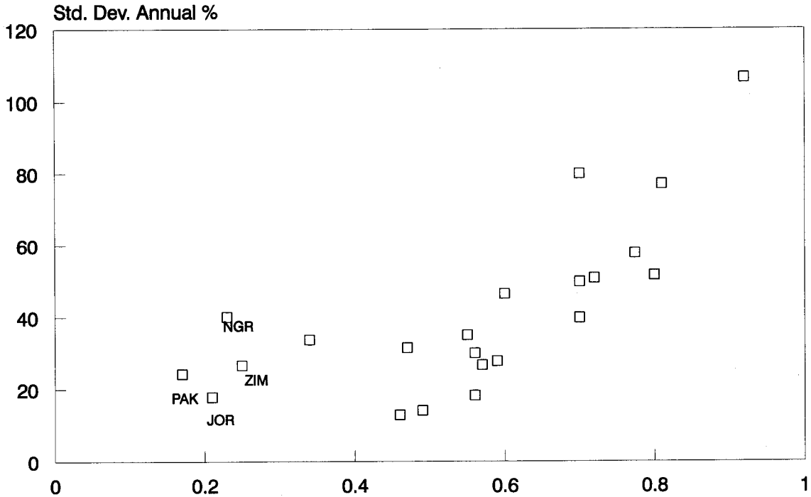
Figure 3: Standard Deviation of Equity Returns and Mean Cross Correlation of Index Stocks
