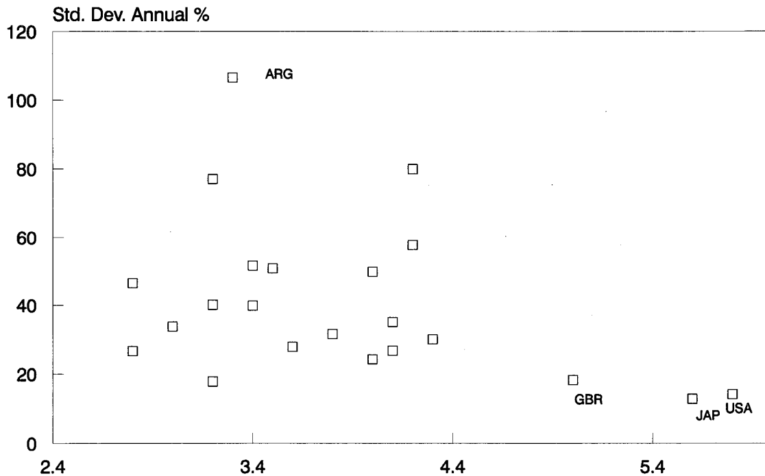
Figure 1: Standard Deviation of Equity Returns and Log Number of Companies in Index
