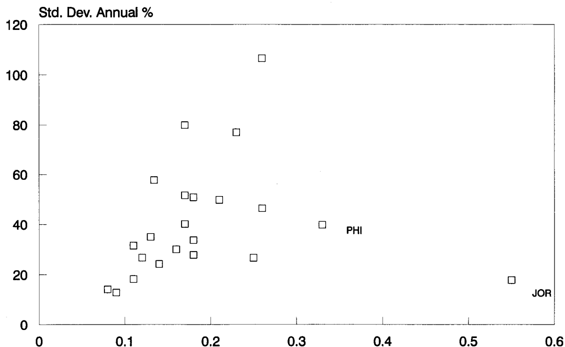
Figure 2: Standard Deviation of Equity Returns and Asset Concentration Factor
