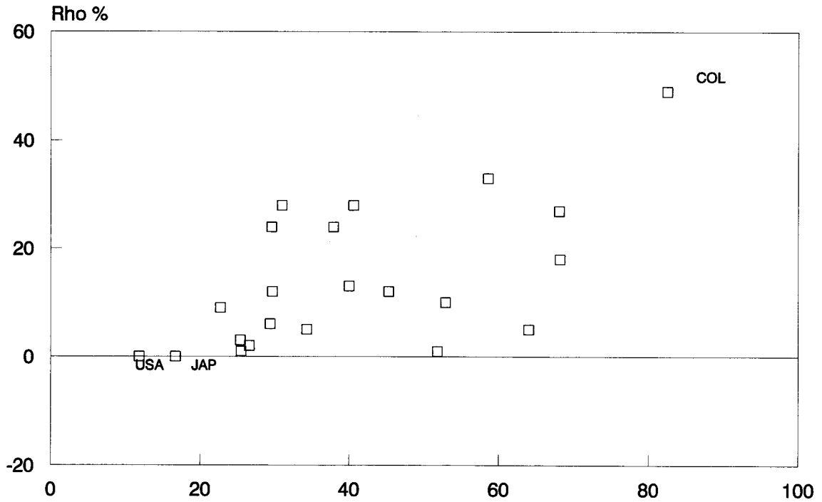
Figure 5: Autocorrelation of Equity Returns Percent Capitalization of Top 10 Firms
