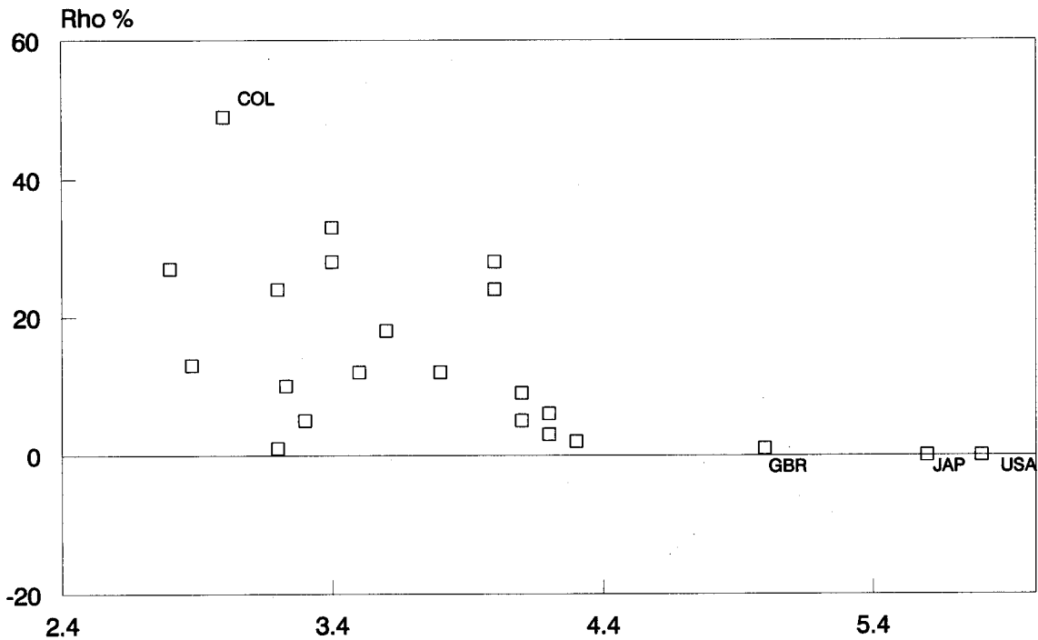
Figure 4: Autocorrelation of Equity Returns Log Number of Companies in Index
