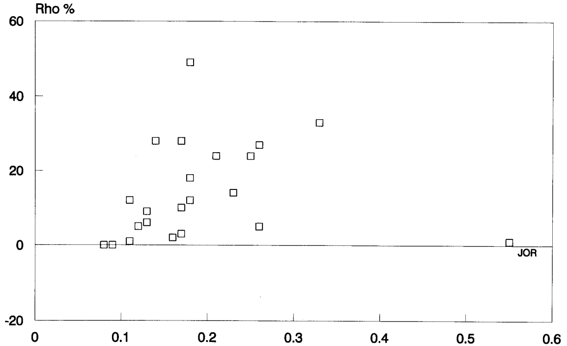
Figure 6: Autocorrelation of Equity Returns Asset Concentration Factor
